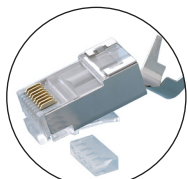
C5e/C6e Shielded RJ45 Connector with Load Bar
